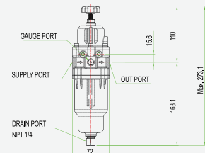
YT-220/YT-225(Auto drain)
